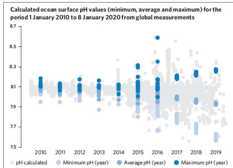
Figure 2. Calculated ocean surface pH values (minimum, average and maximum) for the period 1 January 2010 to 8 January 2020 from global measurements.
