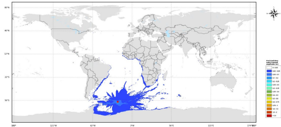
ITEWC Maximum Wave Amplitude Map for South Sandwich Islands
