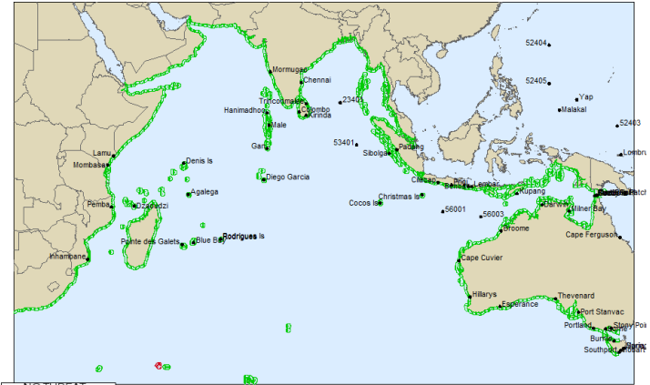
JATWC Threat map for South Sandwich Islands
