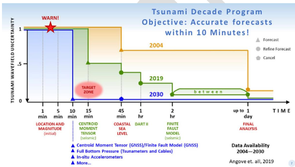
Figure 1: Diagram showing the generalised relationship between tsunami source uncertainty and time after earthquake origin for three different time frames. The orange line represents tsunami source uncertainty levels prior to 2004, the green line represents tsunami source uncertainty levels in 2019, and the blue line represents tsunami source uncertainty levels achievable with the ocean sensing and analysis techniques described in this paper. Initial earthquake location and magnitude is considered “fully uncertain” in terms of solving tsunami source parameters for the purposes of this depiction.
