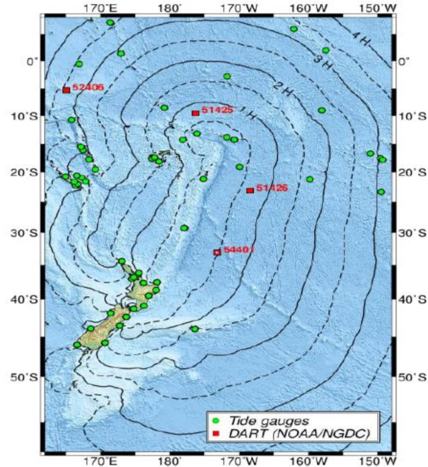
Figure 8. Real-time tide gauge network (green circles) and available deep bottom pressure recorders from the D.A.R.T network (red squares). Minimal tsunami first arrival time isochrons are plotted every 30 mins (dashed black line) and every hour (plain black line) considering the whole Tonga-Kermadec-Hikurangi trench as a tsunami source using Tsunami Travel Times (TTT) software developed by Paul Wessel.
